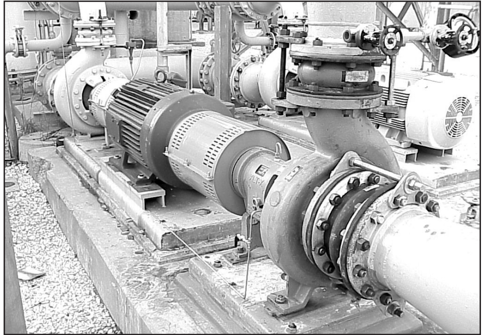
Double shaft extension motor drives the 3196 turbine.
